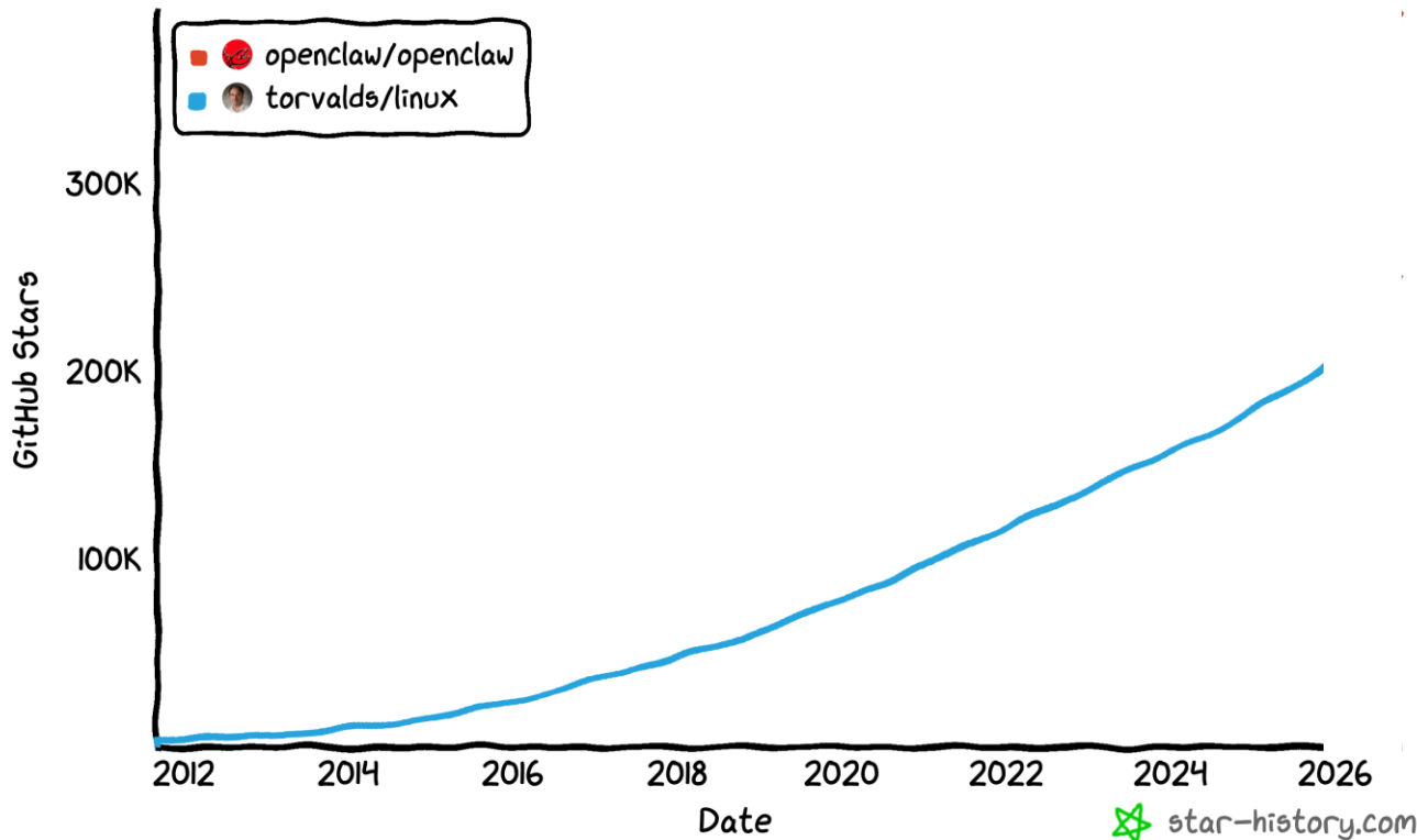
Star History
